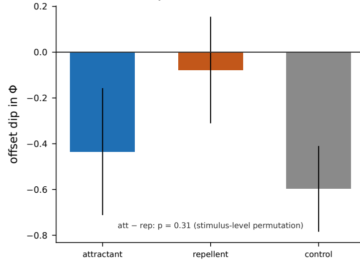
b ...and carries no chemical identity
