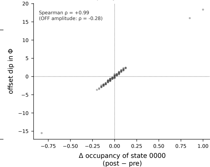
c Mechanism: the dip IS the loss of 0000 occupancy
