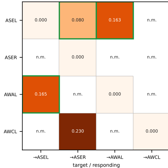
b Effective (signal propagation) (Randi 2023; n.m. = not measured)
