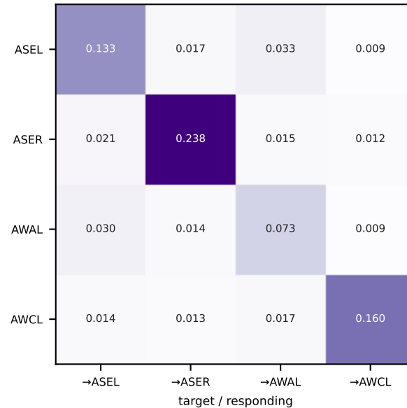
c Ours, full: diagonal dominates the colour scale
