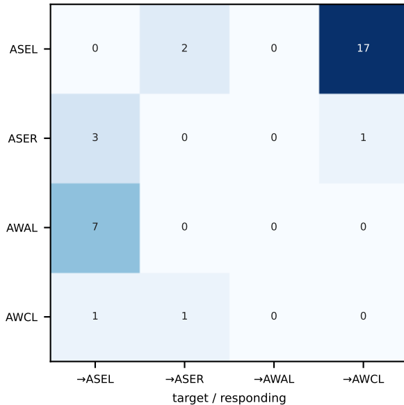
a Anatomy: synaptic contacts (Cook 2019 via OpenWorm)
