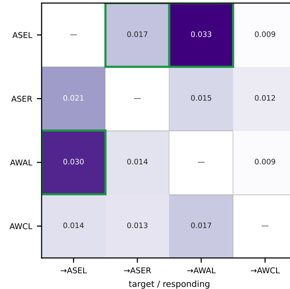
d Ours, diagonal blocked to match b: the cross-pattern emerges
