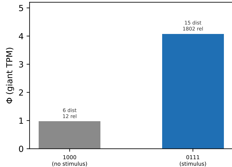
a The two condition states' full-data structures
