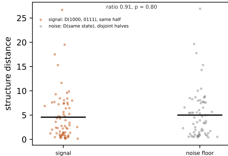
b The comparison fails its noise floor (all 4 variants)
