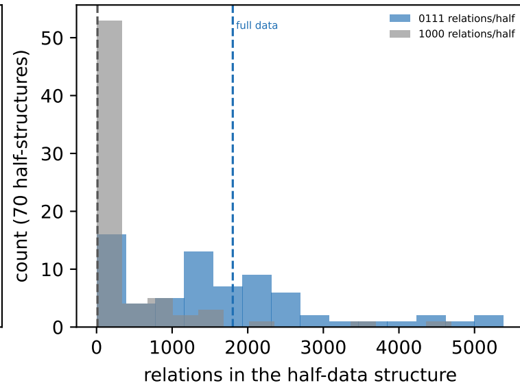
c Why: half-data structures of 0111 swing wildly in size
