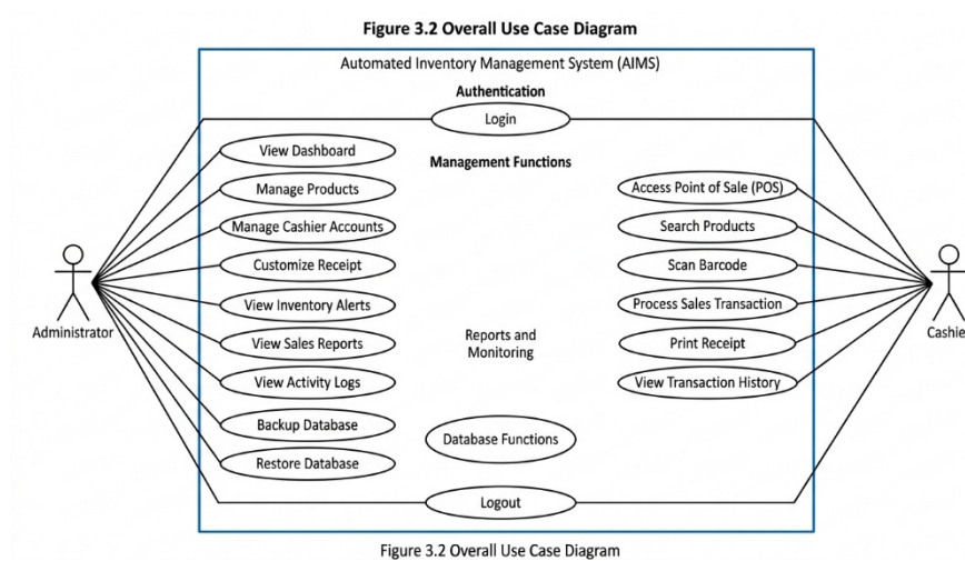
Figure 3.2 Overall Use Case Diagram
