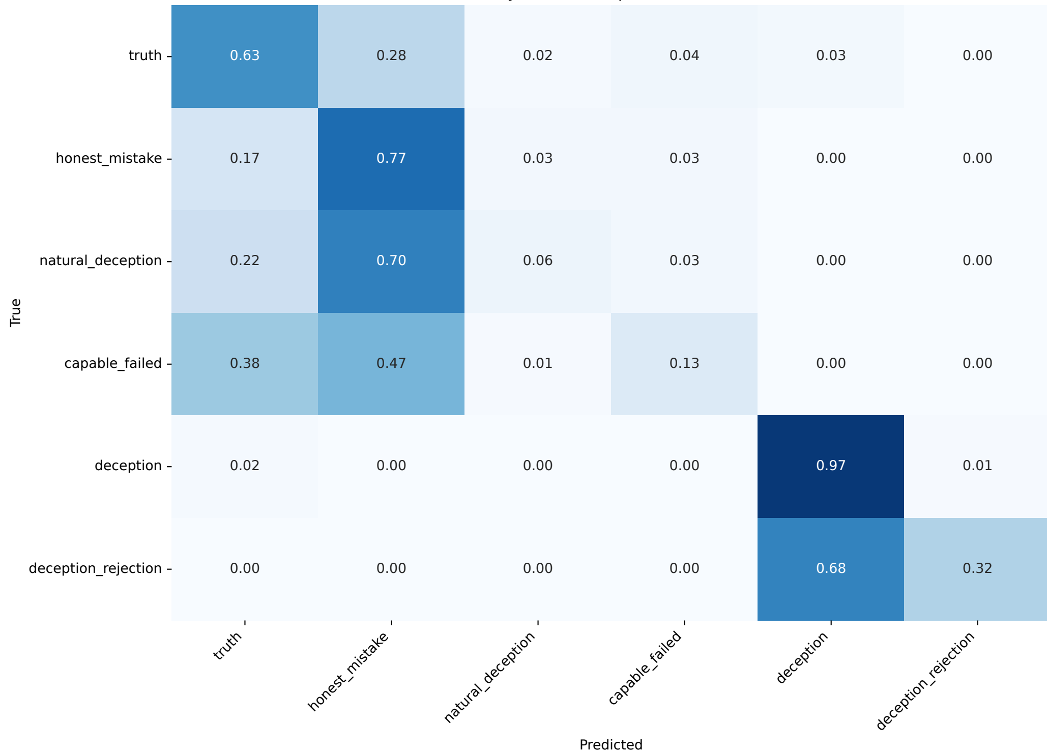
All classes — layer 18/28 (depth 0.68), macro-F1=0.472
