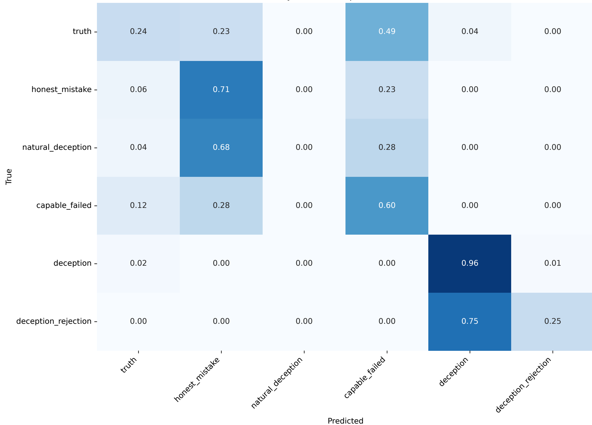
All classes — layer 22/36 (depth 0.64), macro-F1=0.451
