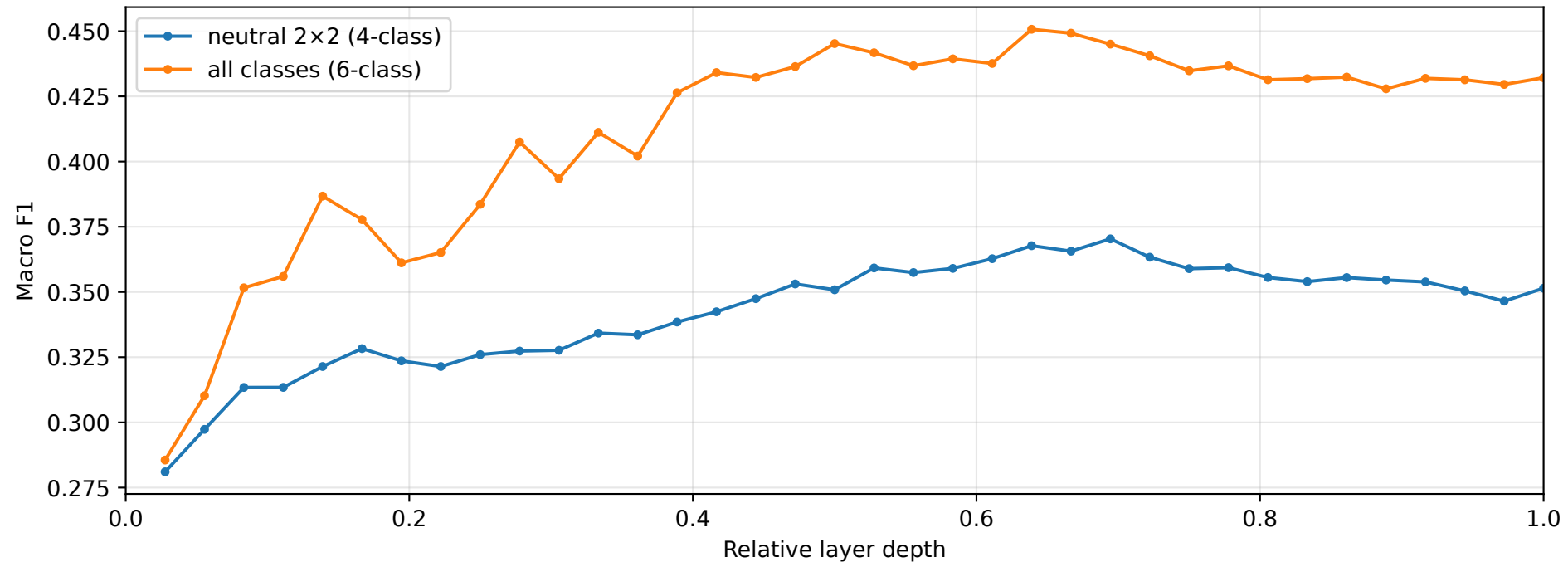
Multiclass probe macro-F1 by layer depth
