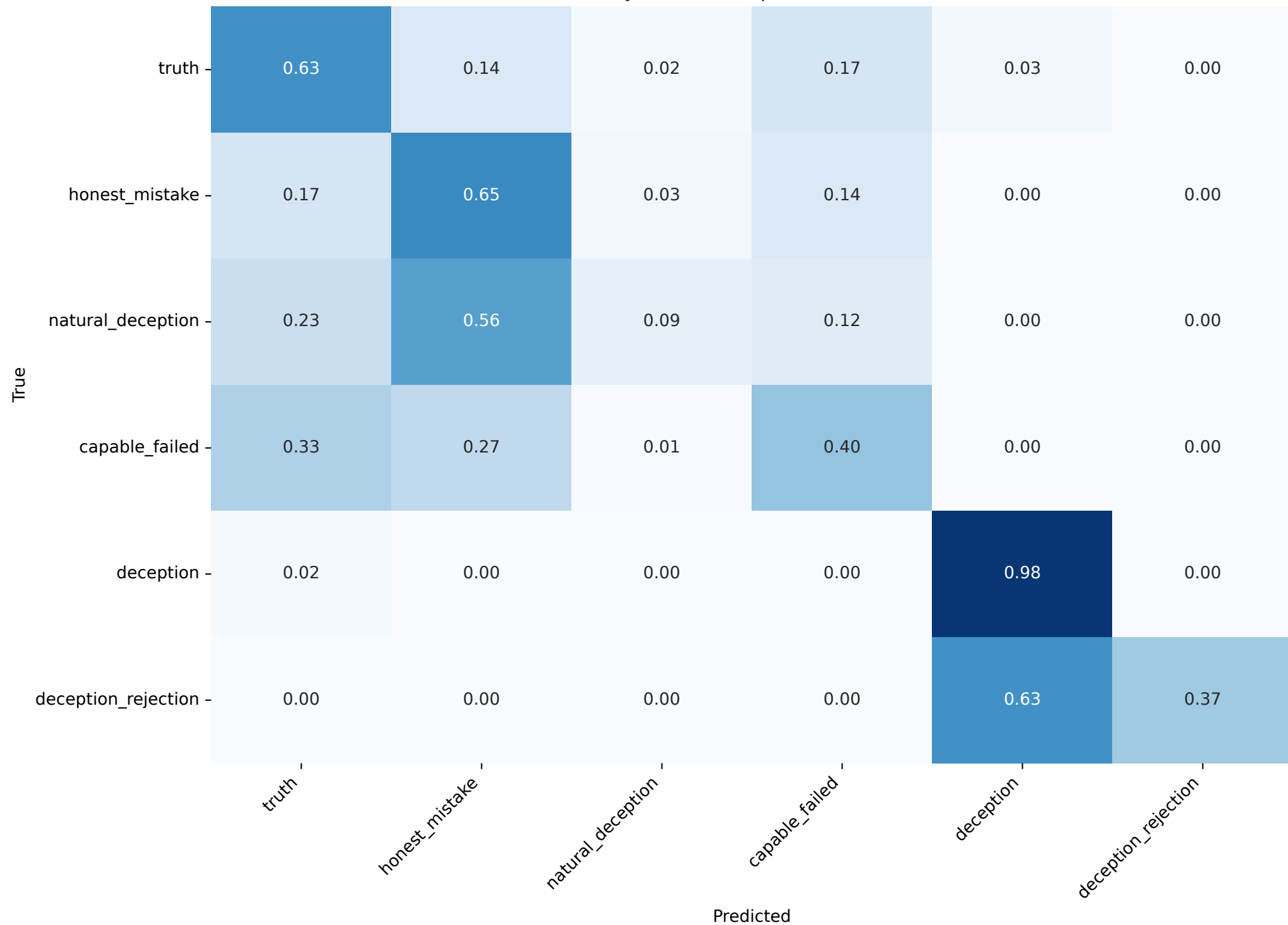
All classes — layer 25/42 (depth 0.62), macro-F1=0.528
