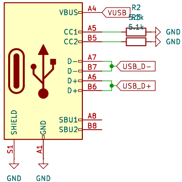
USB-C Port USB_C_Receptacle_USB2.0_16P
