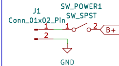
Battery Connector and Power Switch
