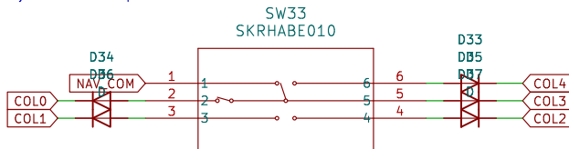
5 way nav switch – part of switch matrix
