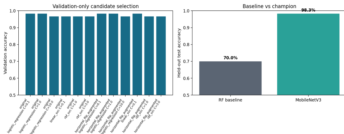
Figure 1. Held-out comparison of the preserved random-forest baseline and the MobileNetV3 champion. Accuracy rises from 70.00% to 98.33%, a 28.33 percentage-point gain.
