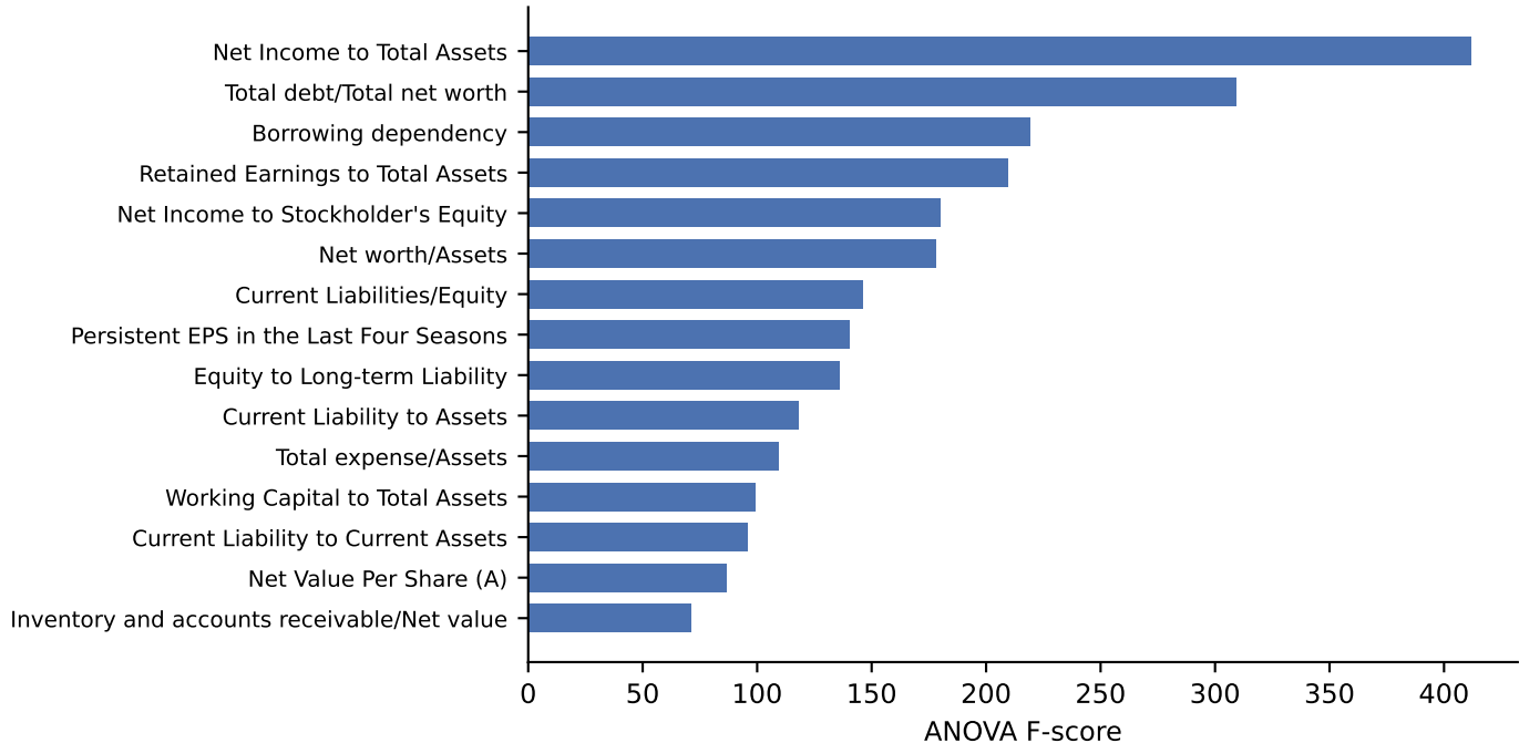
Top 15 features by ANOVA F-test
