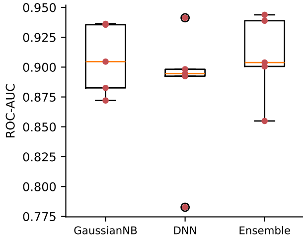
ROC-AUC across 5 folds
