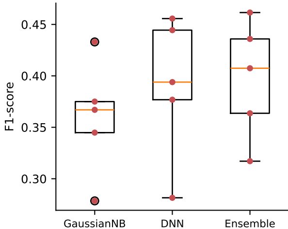
F1-score across 5 folds
