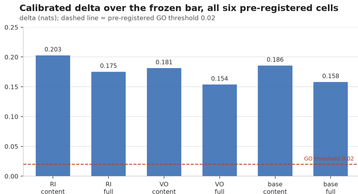
Figure 1. Calibrated delta over the frozen model-free bar, all six pre-registered cells (v2, 8,000 claims, all fits frozen from v1).
