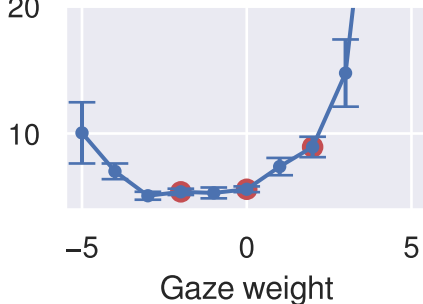
Readability (FKGL)
