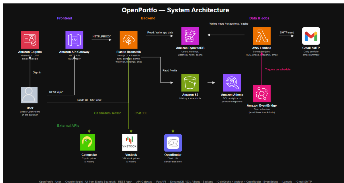
Figure 1. OpenPortfo high-level architecture.
