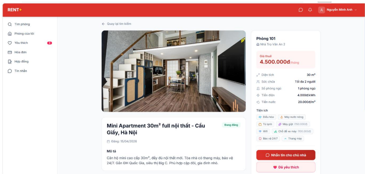
Figure 3. Boarding house details page for tenants.
