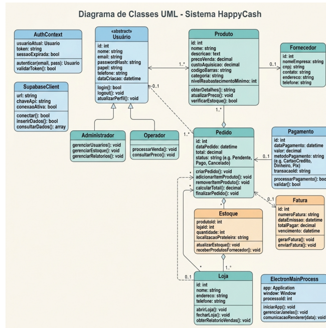
Figure 1: Diagrama de Classes
