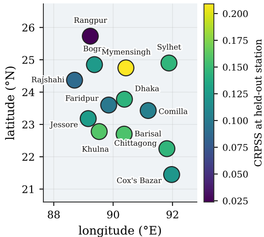
(b) LOSO transfer skill (h=2)
