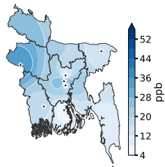
(c) \text{NO}_2 surface
