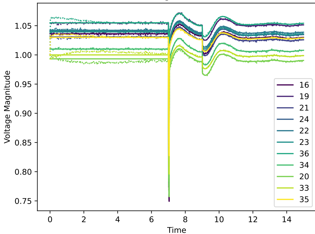
Voltage Profiles
