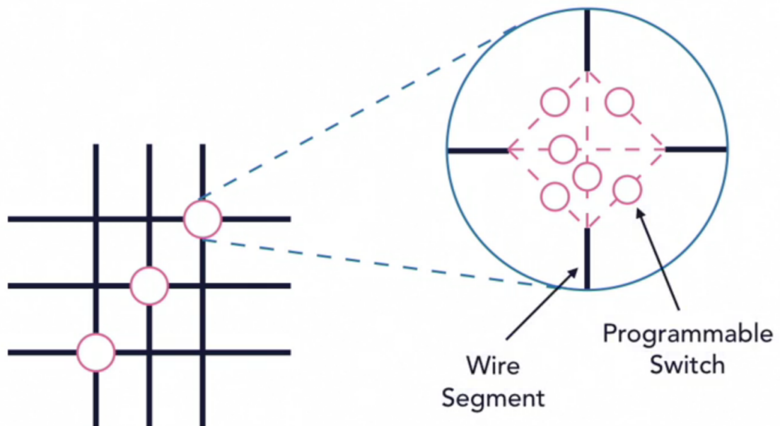
Figure 5: Switch Box
