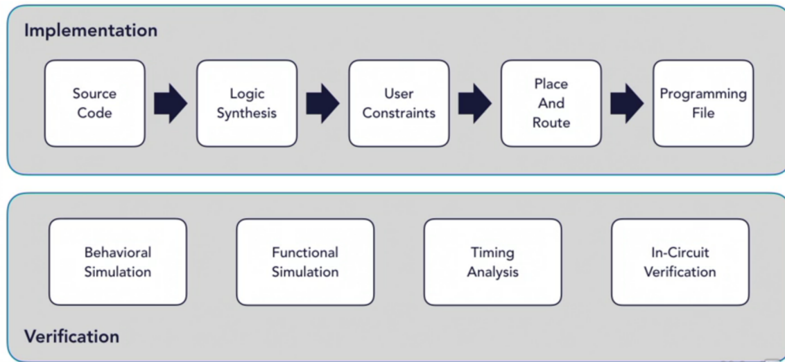
Figure 6: FPGA development process
