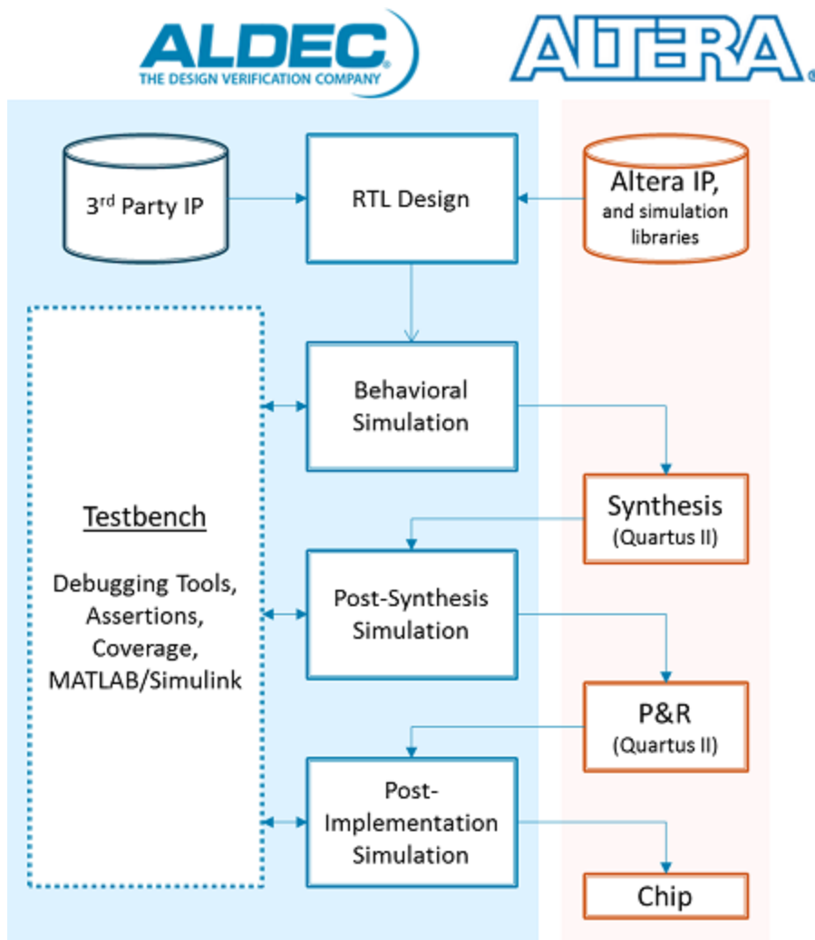
Figure 8: Intel / Altera FPGA development process
