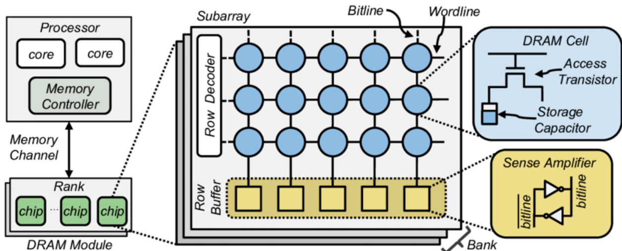
Figure 5: Organization of the DRAM
