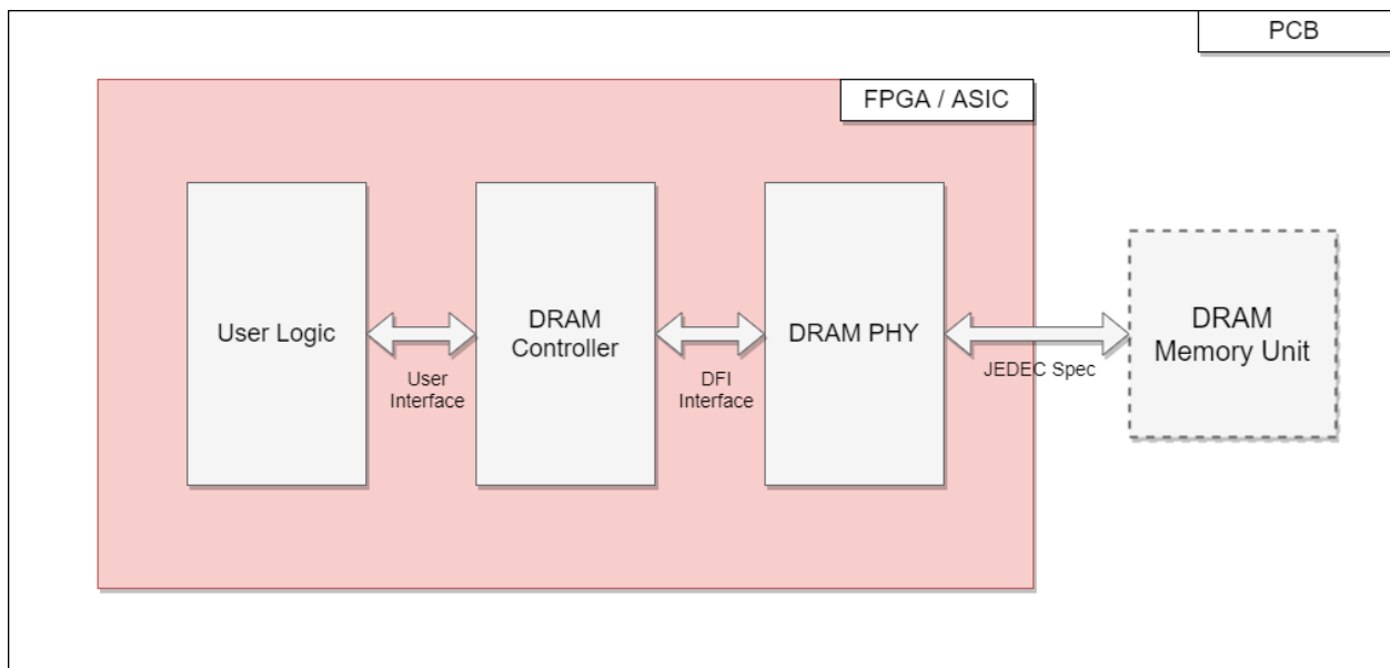
Figure 6: DRAM Subsystem
