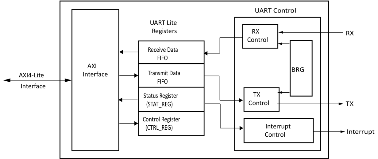
Figure 1: Internal block diagram of AXI UART IP
