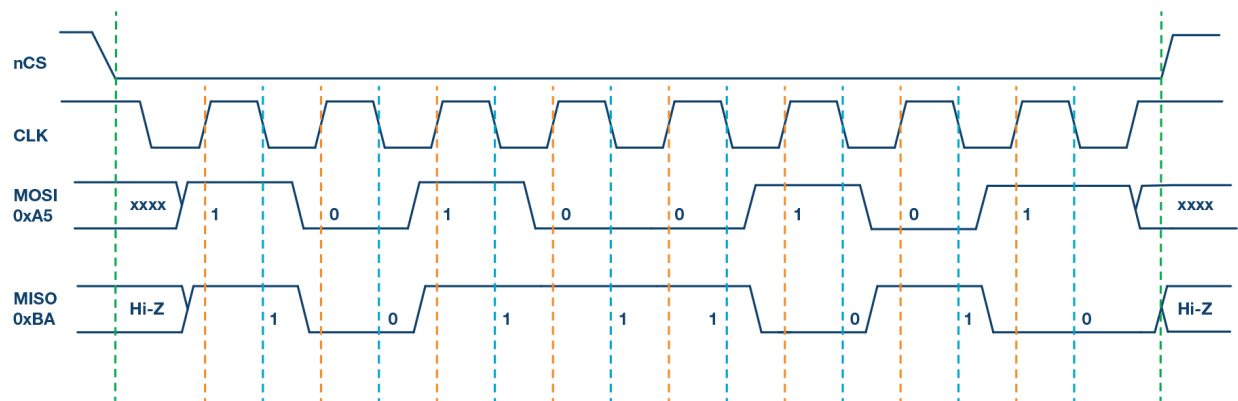
Figure 8: SPI Mode 3, CPOL = 1, CPHA = 0: CLK idle state = high, data sampled on the rising edge and shifted on the falling edge.
