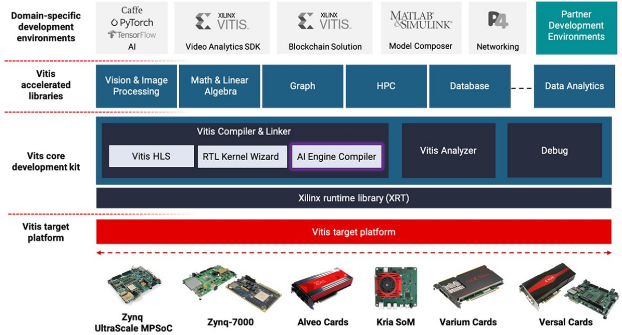
Figure 1: Vitis Unified Software Platform Overview
