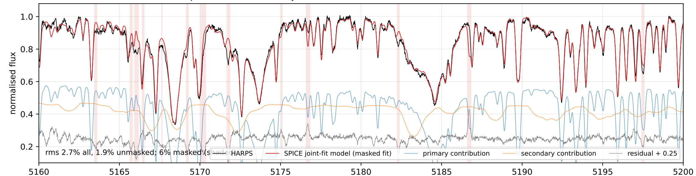
TZ For at phase 0.25: masked joint fit (Teff1 4898 K, Teff2 6366 K, [Fe/H] -0.18) vs HARPS
