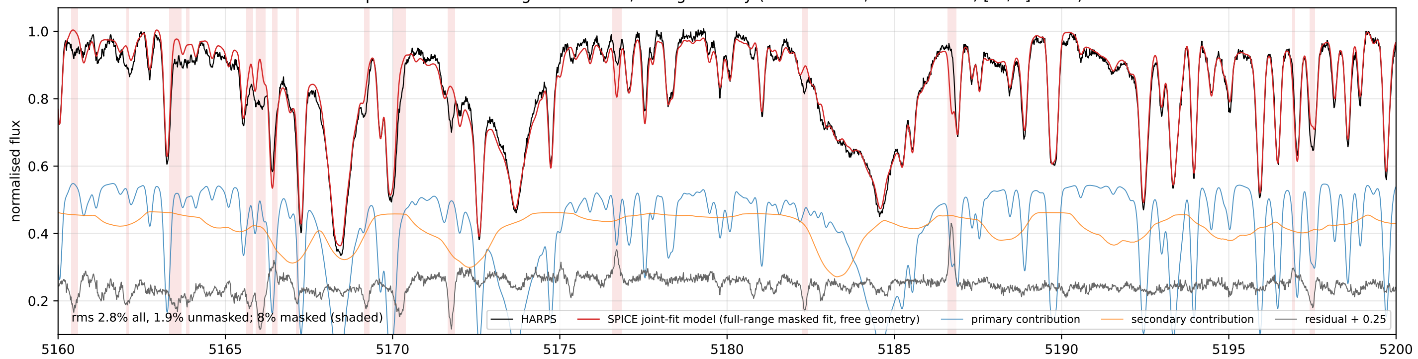
TZ For at phase 0.25: full-range masked fit, free geometry (Teff1 4904 K, Teff2 6275 K, [Fe/H] -0.17) vs HARPS
