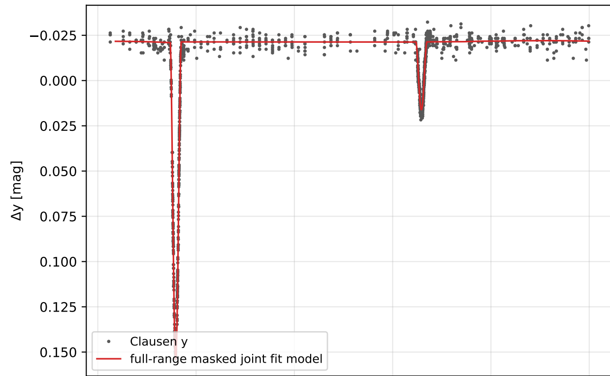
TZ For Strömgren b, y: Clausen photometry vs the full-range masked joint fit model
