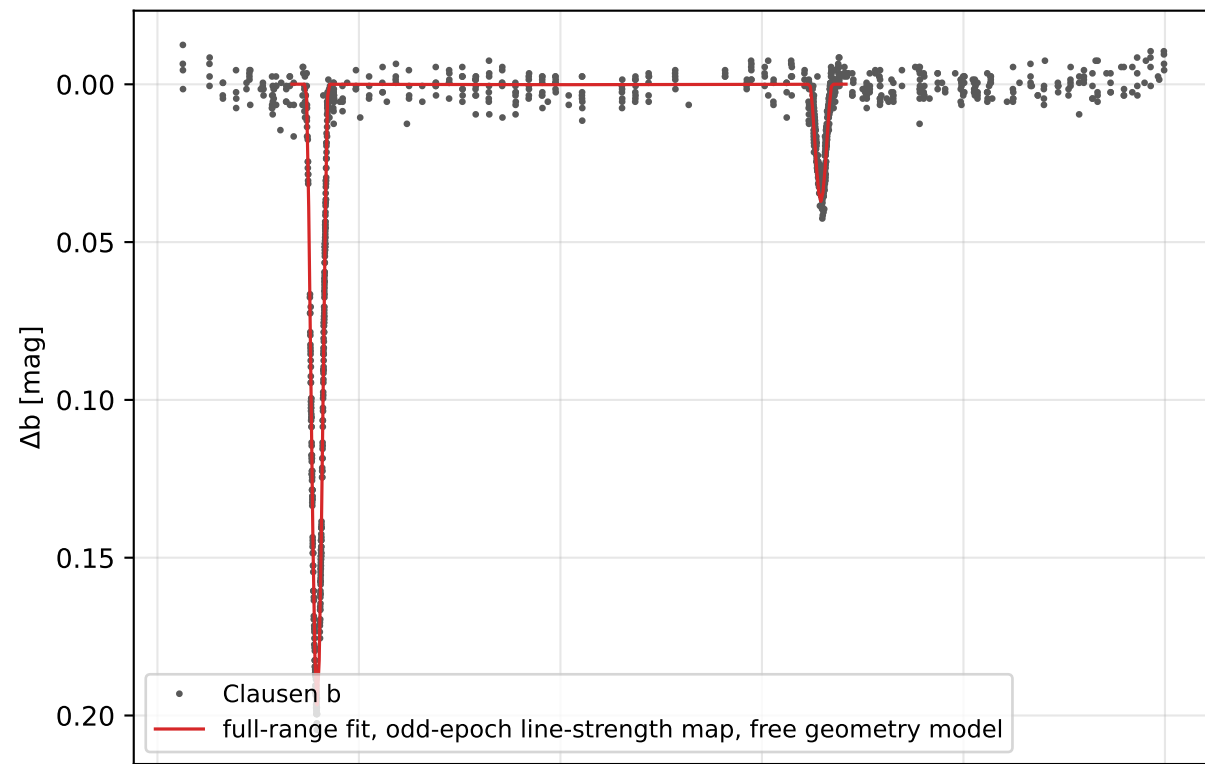
TZ For Strömgren b, y: Clausen photometry vs the full-range fit, odd-epoch line-strength map, free geometry model
