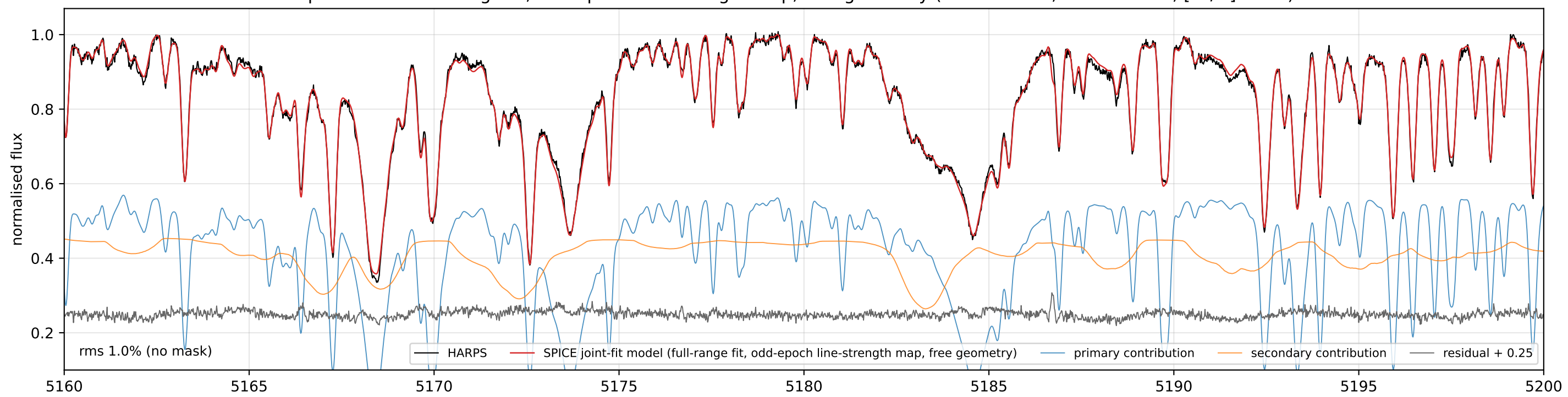
TZ For at phase 0.25: full-range fit, odd-epoch line-strength map, free geometry (Teff1 4879 K, Teff2 6211 K, [Fe/H] -0.27) vs HARPS
