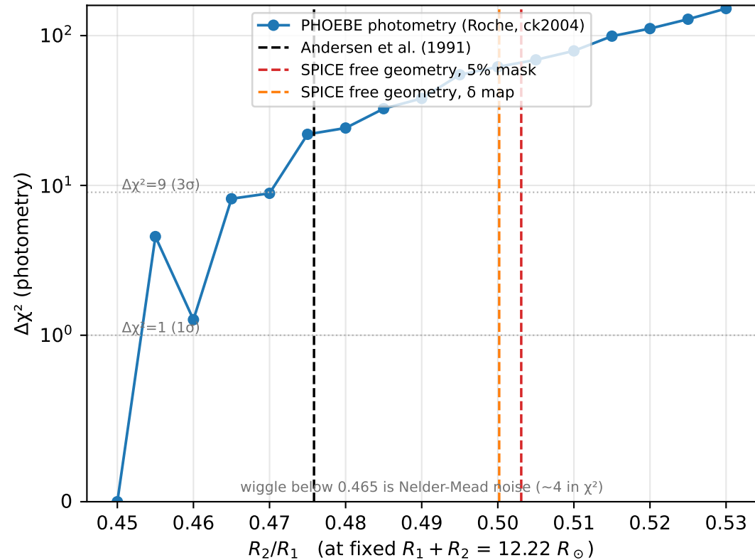
The photometry's constraint on the radius ratio (inclination fixed)
