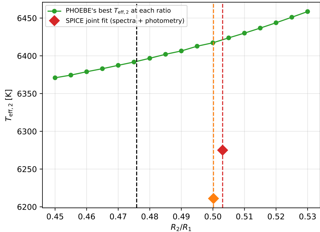
Size and temperature trade off at fixed eclipse depth
