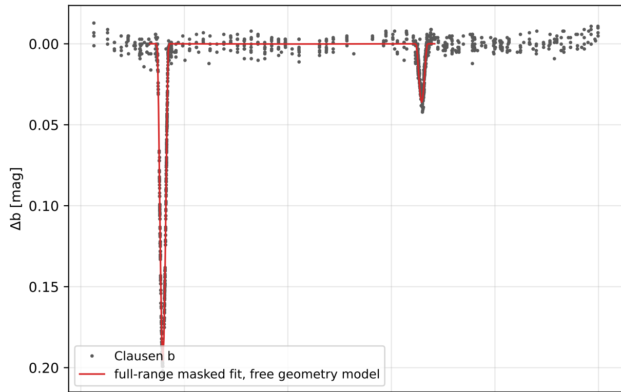
TZ For Strömgren b, y: Clausen photometry vs the full-range masked fit, free geometry model
