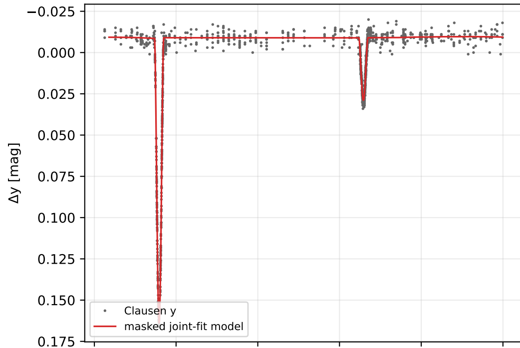
TZ For Strömgren b, y: Clausen photometry vs the masked joint-fit model
