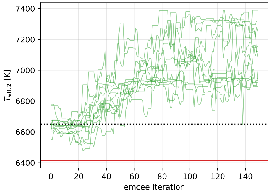
PHOEBE-native emcee on b, y photometry: walkers drift along the degenerate ridge (corr = +1.000)
