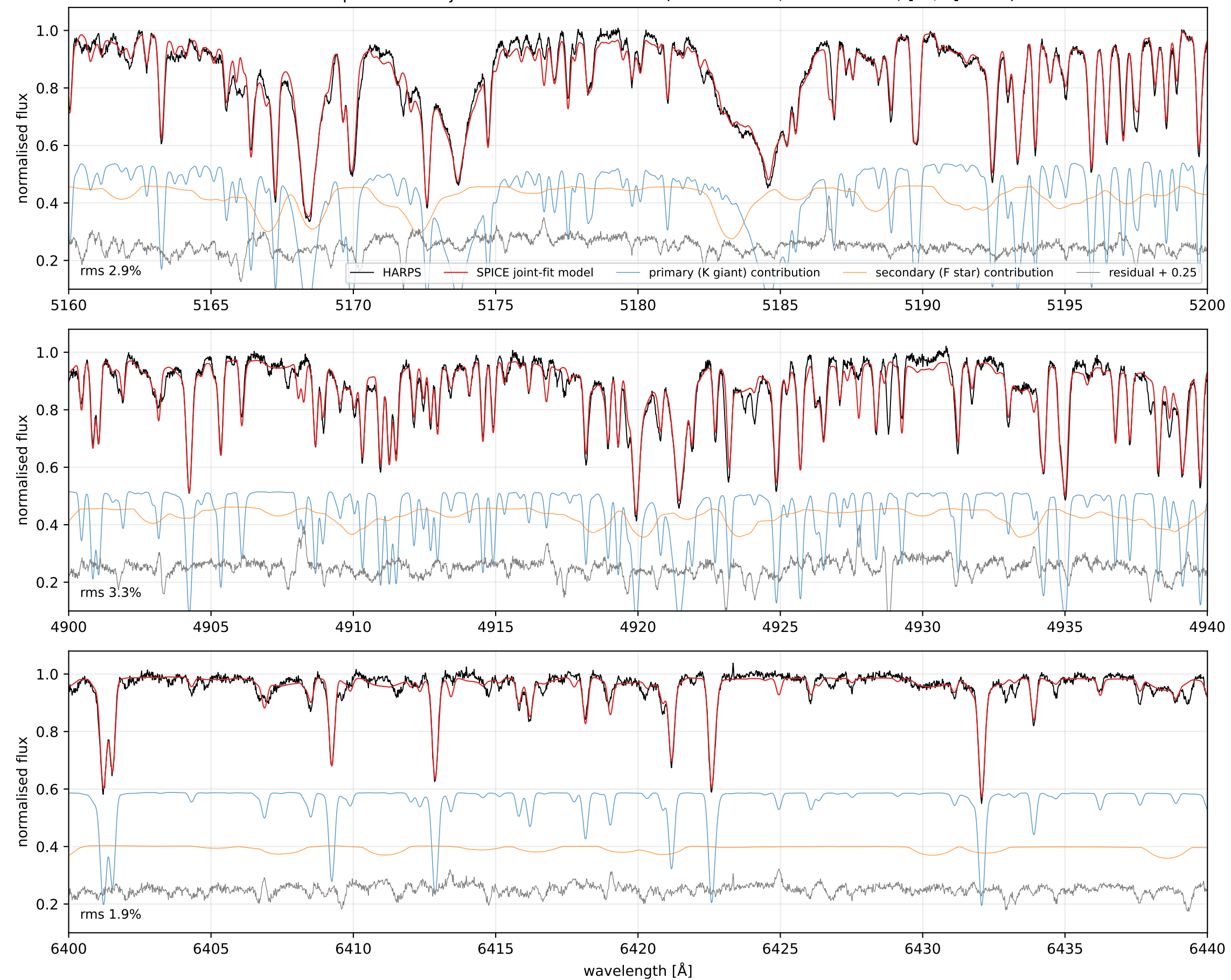
TZ For at phase 0.25: joint-fit model vs HARPS (Teff1 4889 K, Teff2 6416 K, [Fe/H] -0.23)
