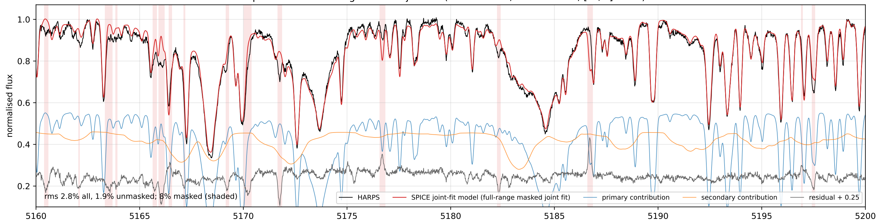
TZ For at phase 0.25: full-range masked joint fit (Teff1 4896 K, Teff2 6396 K, [Fe/H] -0.17) vs HARPS
