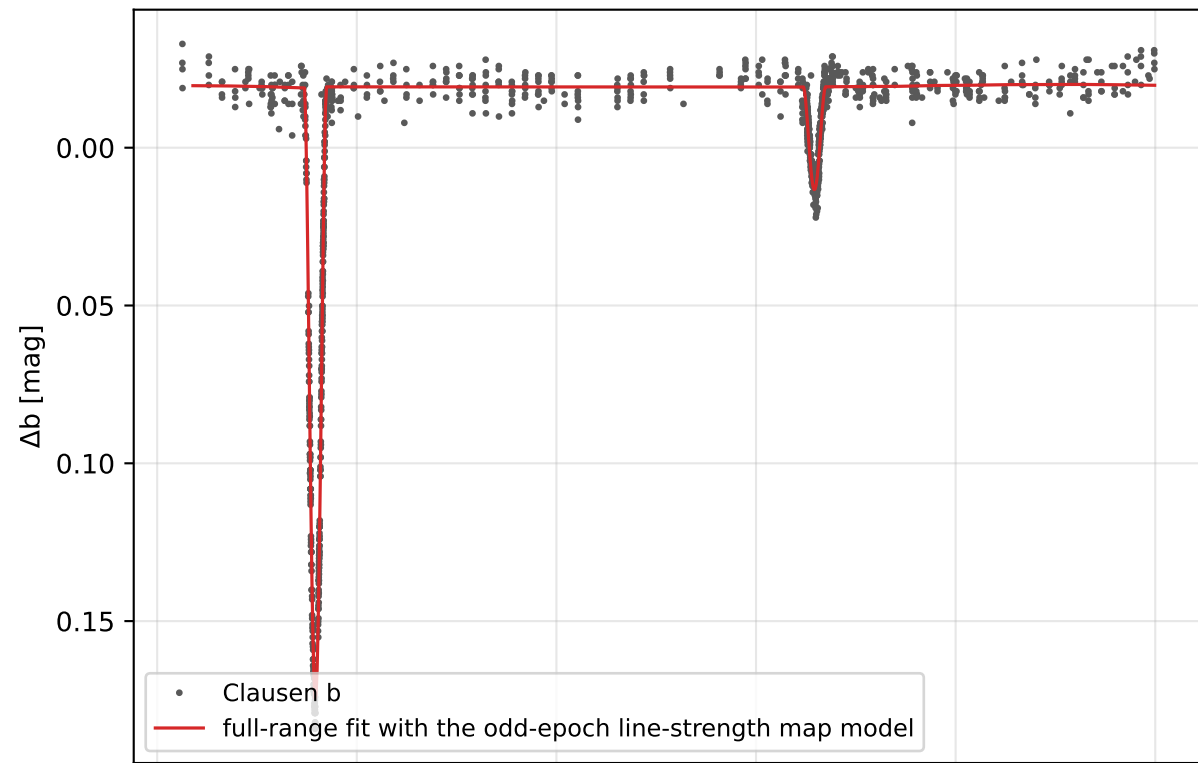
TZ For Strömgren b, y: Clausen photometry vs the full-range fit with the odd-epoch line-strength map model
