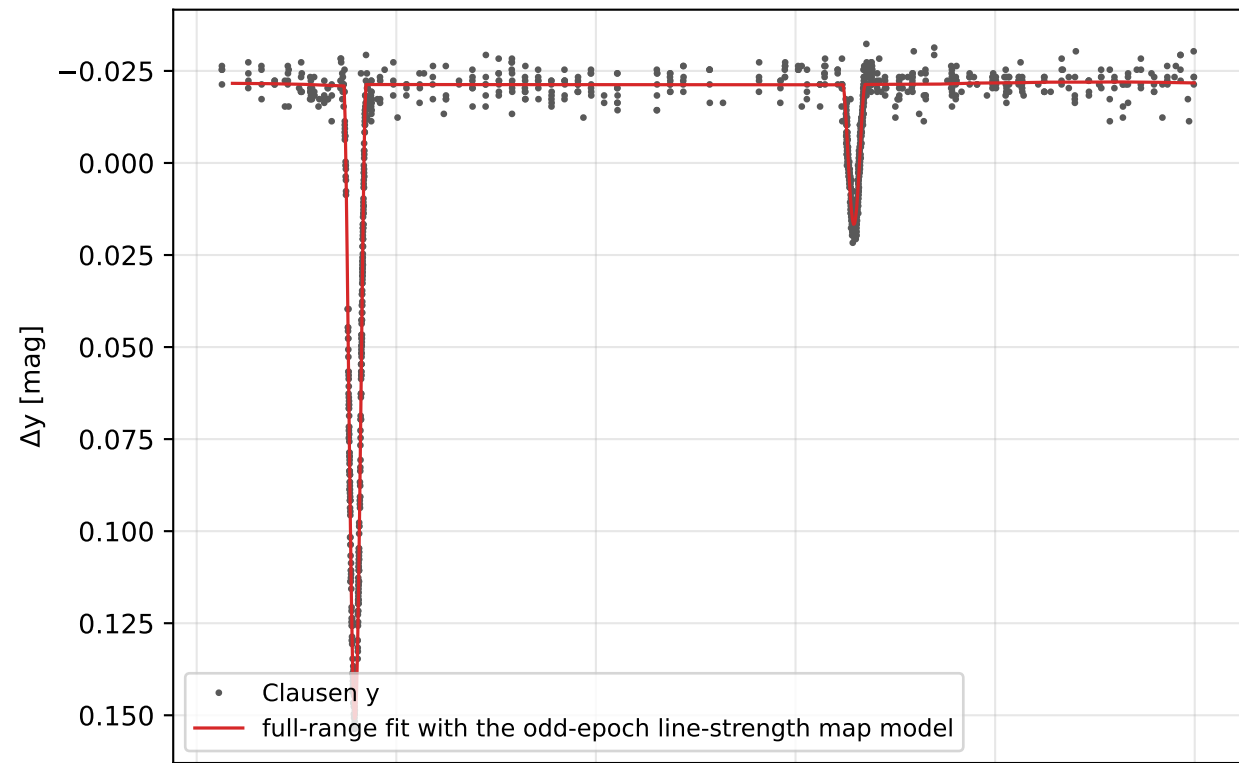
TZ For Strömgren b, y: Clausen photometry vs the full-range fit with the odd-epoch line-strength map model
