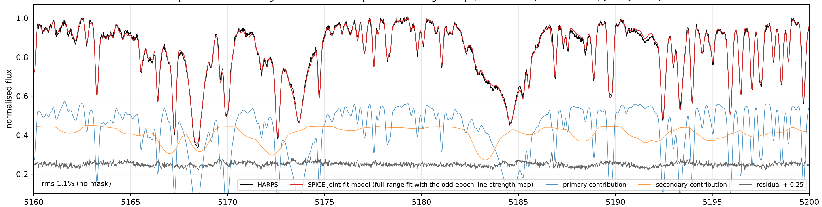
TZ For at phase 0.25: full-range fit with the odd-epoch line-strength map (Teff1 4874 K, Teff2 6319 K, [Fe/H] -0.27) vs HARPS
