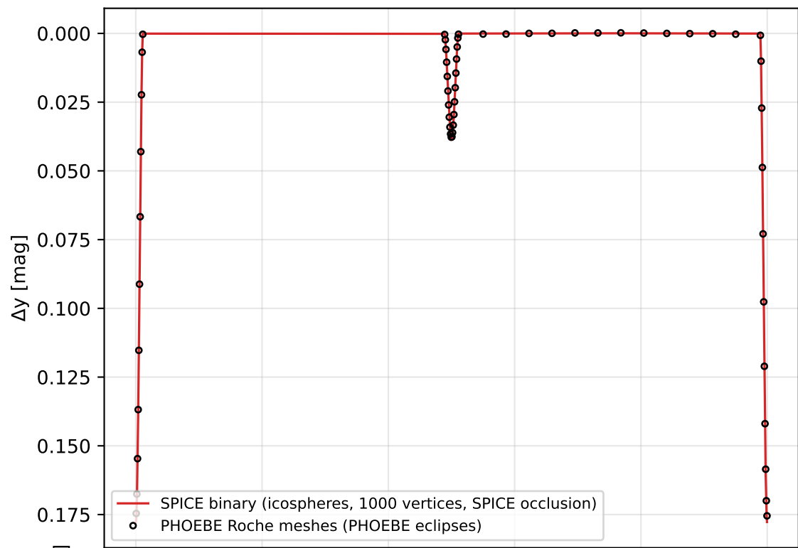
TZ For Strömgren b, y at the best-fit temperatures: SPICE's own binary vs the PHOEBE meshes, same emulator and kernels
