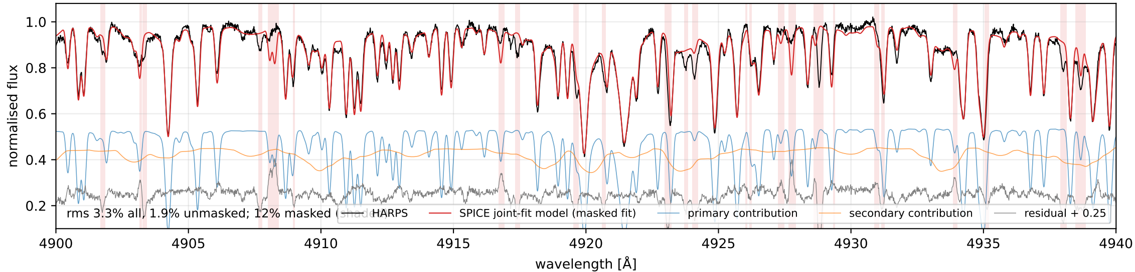
TZ For at phase 0.25: masked joint fit (Teff1 4898 K, Teff2 6366 K, [Fe/H] -0.18) vs HARPS
