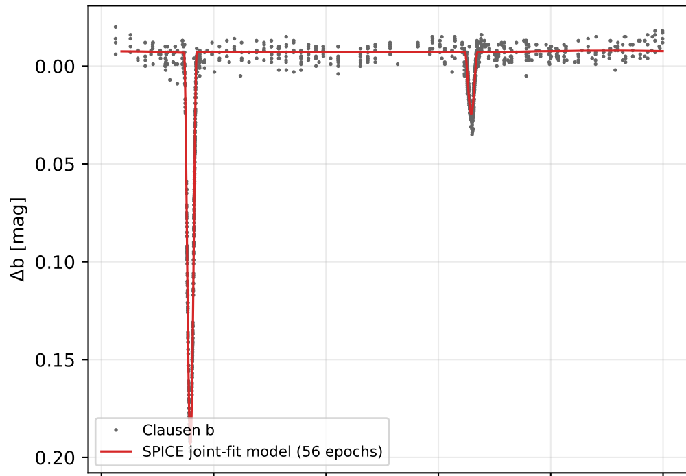
TZ For Strömgren b, y: Clausen photometry vs the joint-fit model
