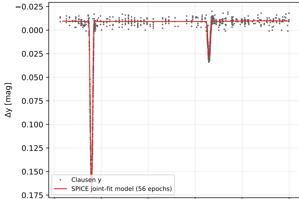
TZ For Strömgren b, y: Clausen photometry vs the joint-fit model
