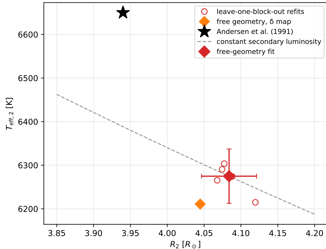
The secondary's light, split between size and temperature
