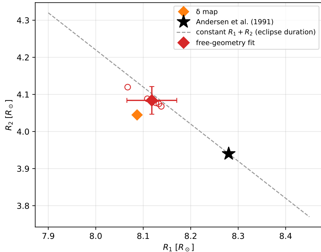
Radii: the sum is fixed, the ratio is not
