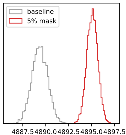
NUTS posteriors on the frozen emulator grid (statistical widths only: \sim 1 K, 0.001 dex)
