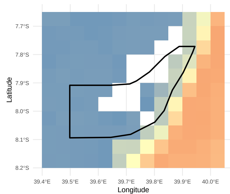
SSP5–8.5 (2060)
