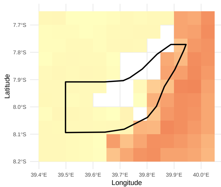
SSP5–8.5 (2070)
