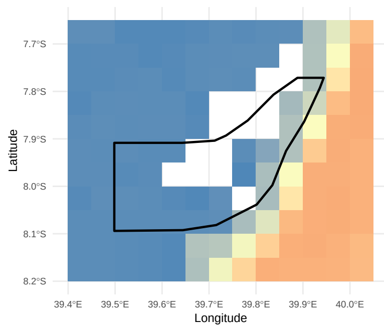
SSP5–8.5 (2050)
