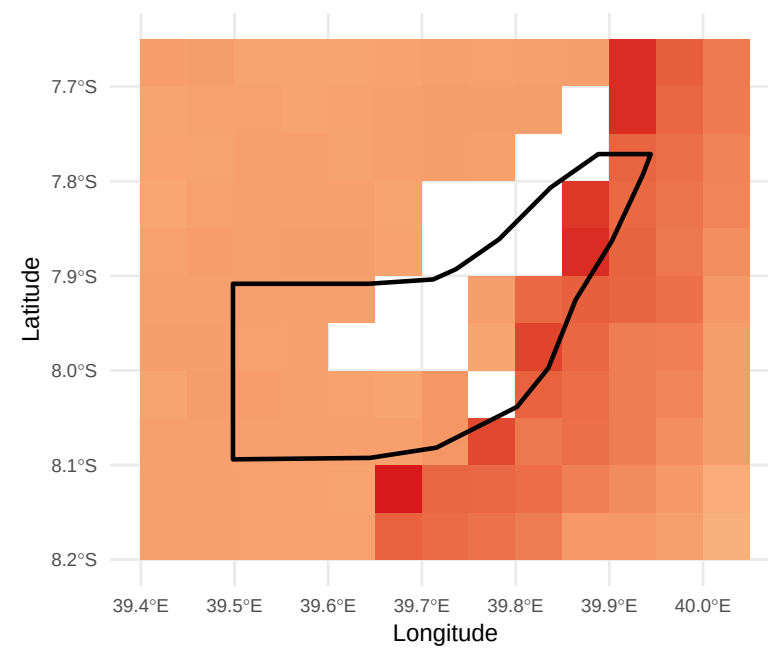
SSP5–8.5 (2090)
