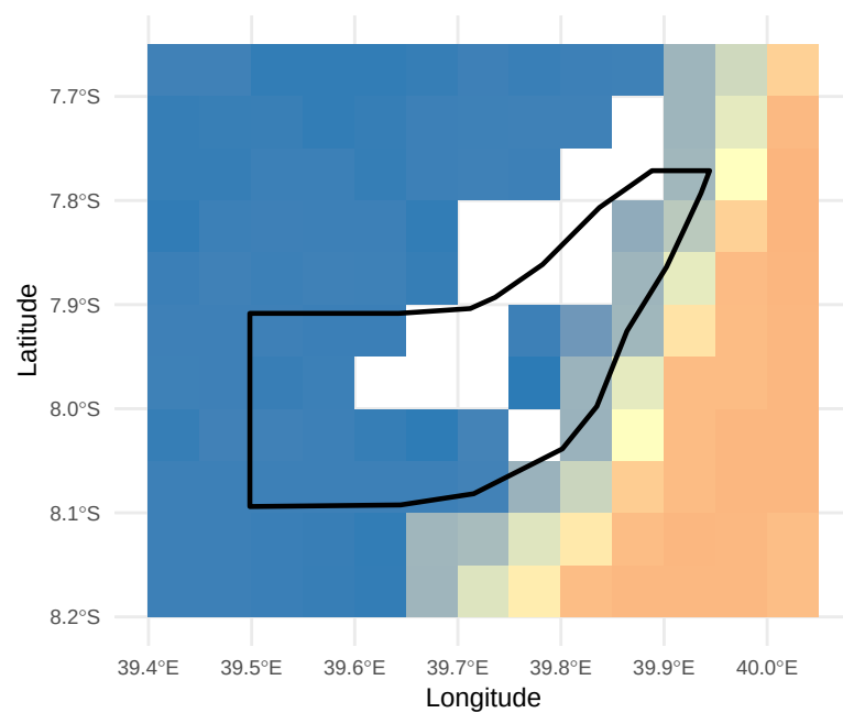
SSP5–8.5 (2040)
