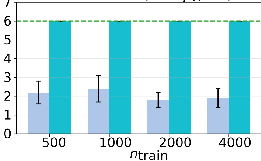
mediator-9x2 (true p_h = 2 )
