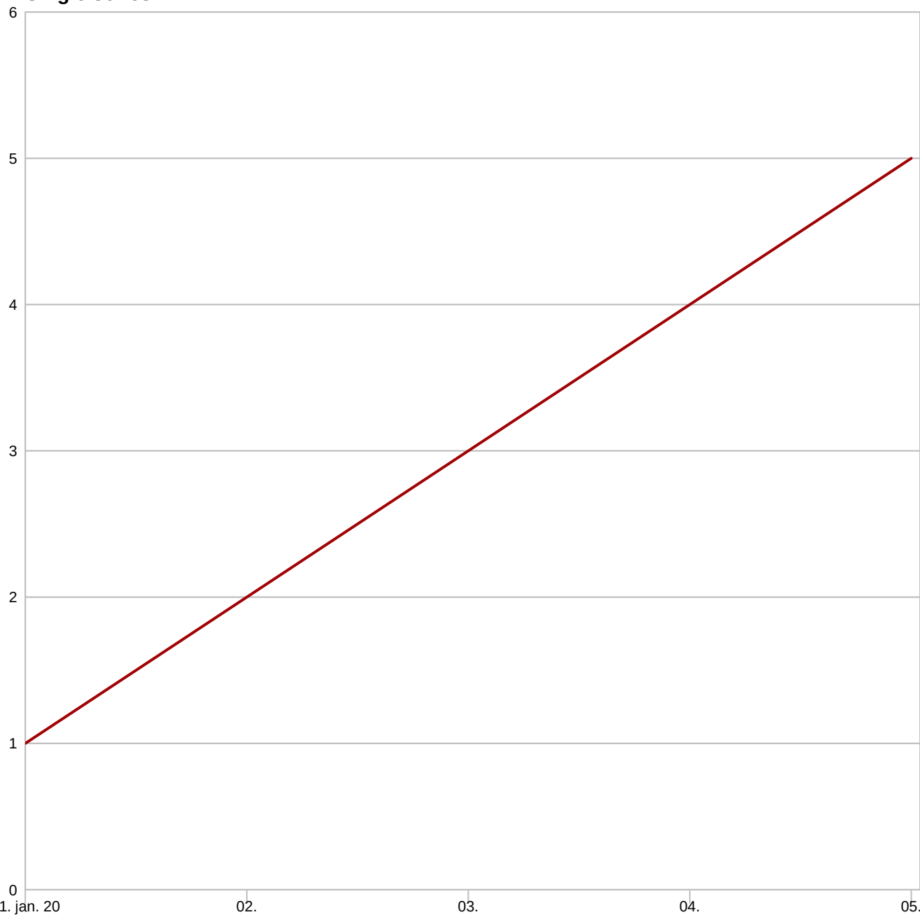
Single series
