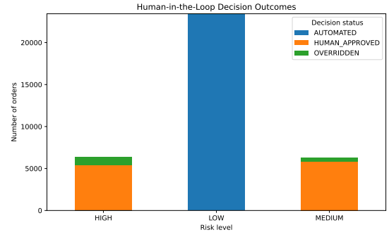
Figure 9: Simulated human-review decisions across the operational risk levels.
