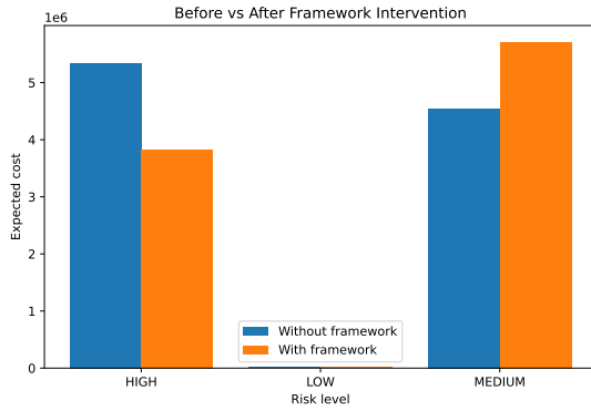
Figure 10: Estimated baseline and decision-policy costs under the primary cost scenario.
