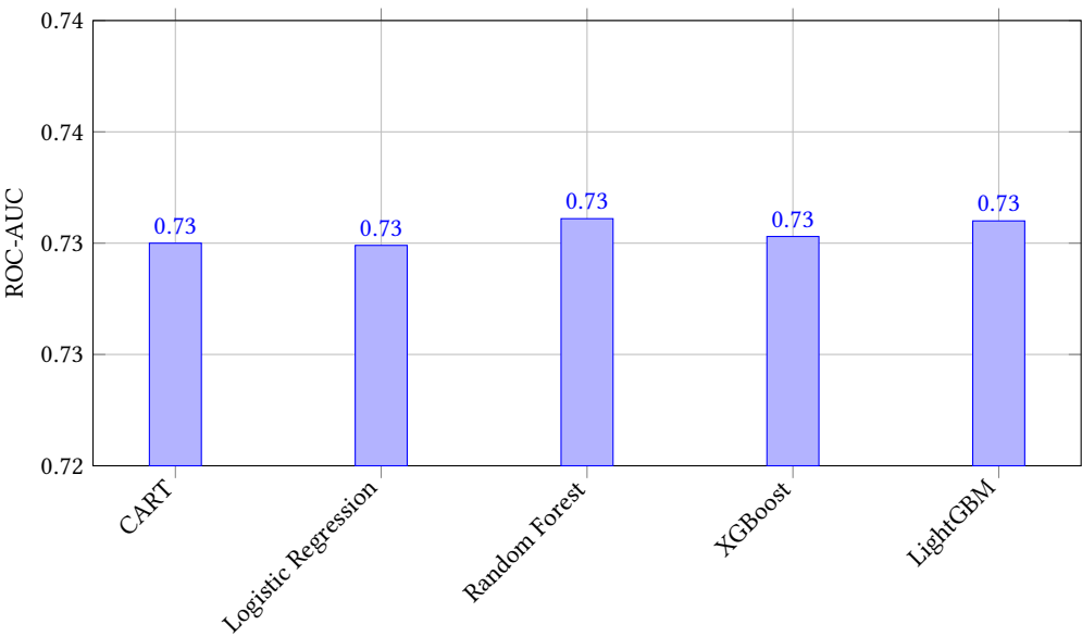
Fig. 4. Comparison of predictive model performance using ROC-AUC.
