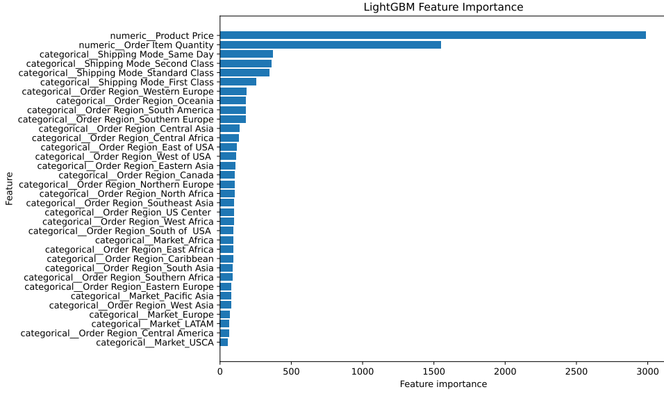
Fig. 6. Feature importance analysis of the selected LightGBM classifier for late-delivery risk prediction.
