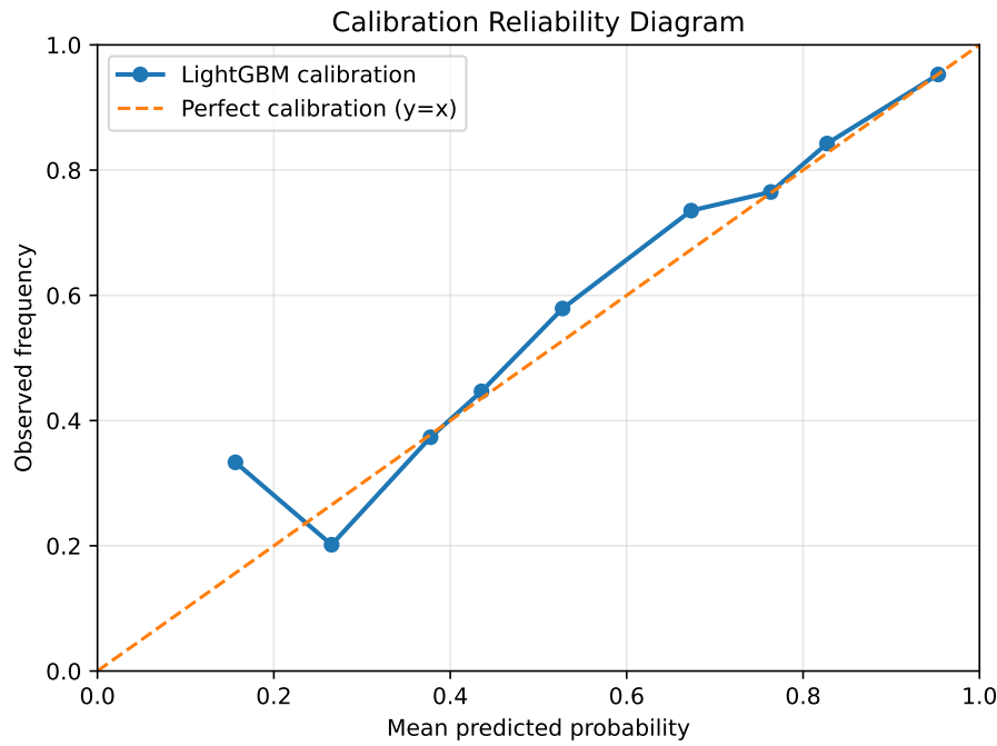
Fig. 8. Probability calibration curve of the selected LightGBM model on the held-out test set.
