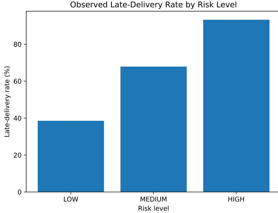
Fig. 7. Observed late-delivery rates across predefined risk categories.
