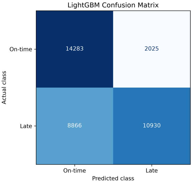
Fig. 5. Confusion matrix of the selected LightGBM classifier on the held-out test set.
