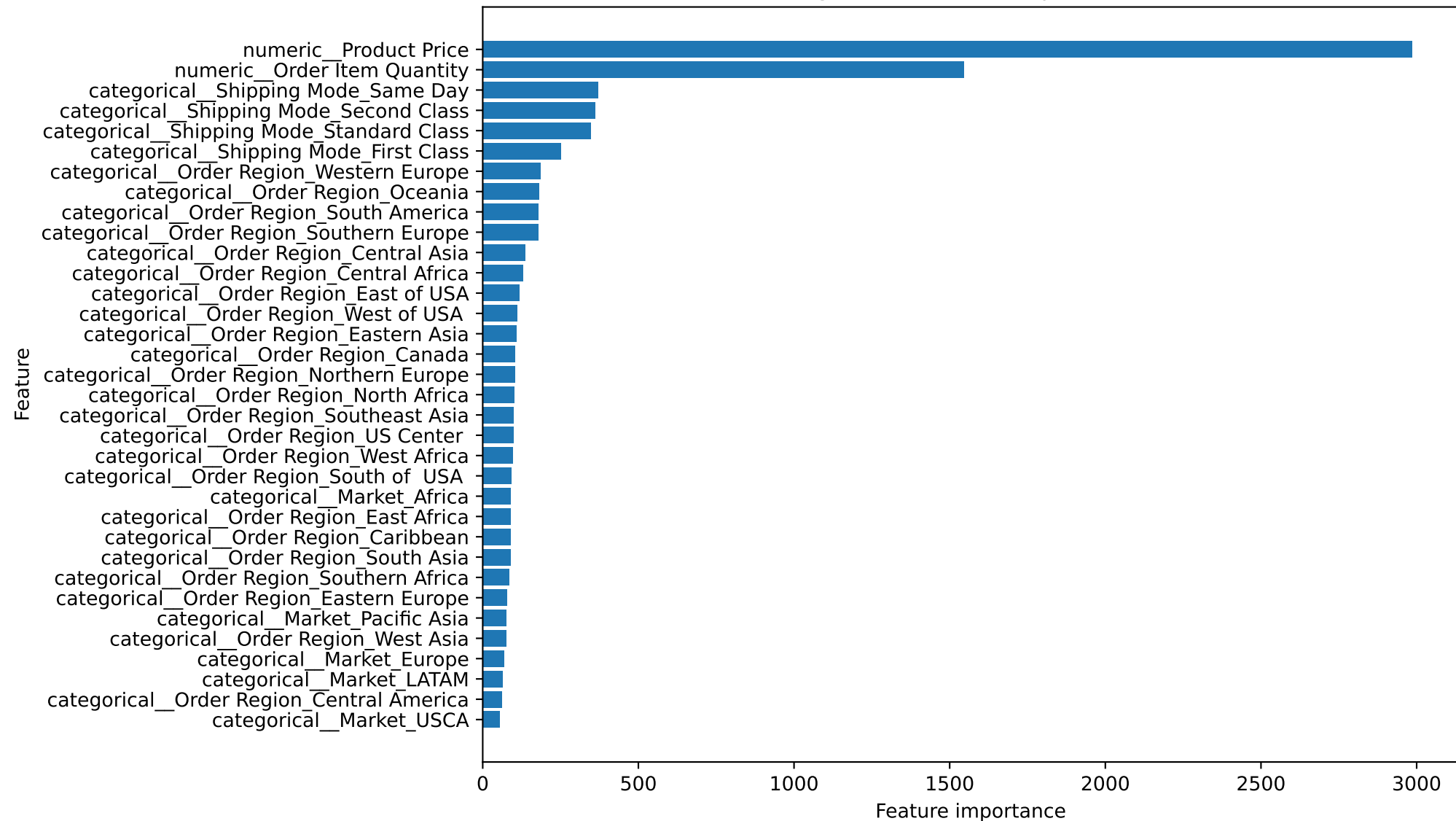
LightGBM Feature Importance
