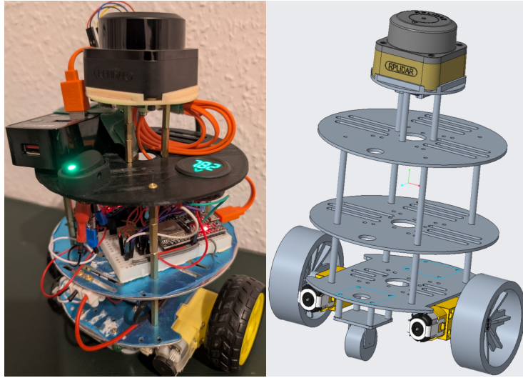
Figure 1: verwendete Roboter
