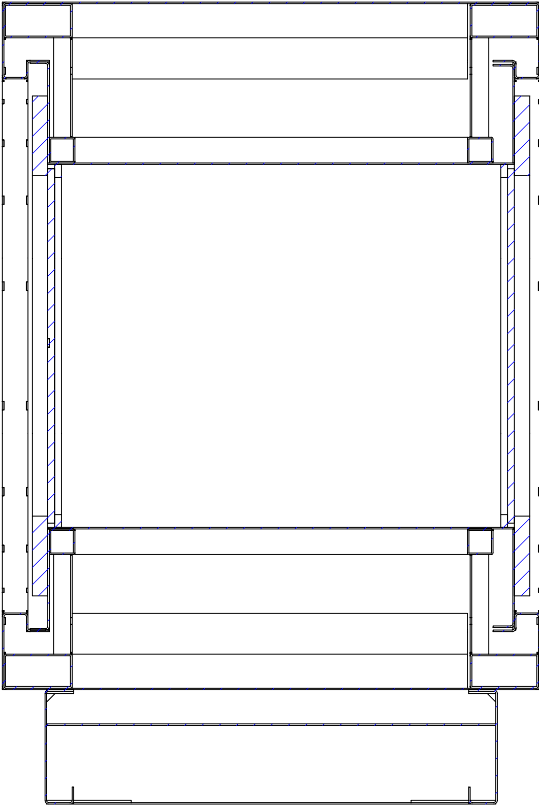
SECTION M-M SCALE 1 : 4.5
